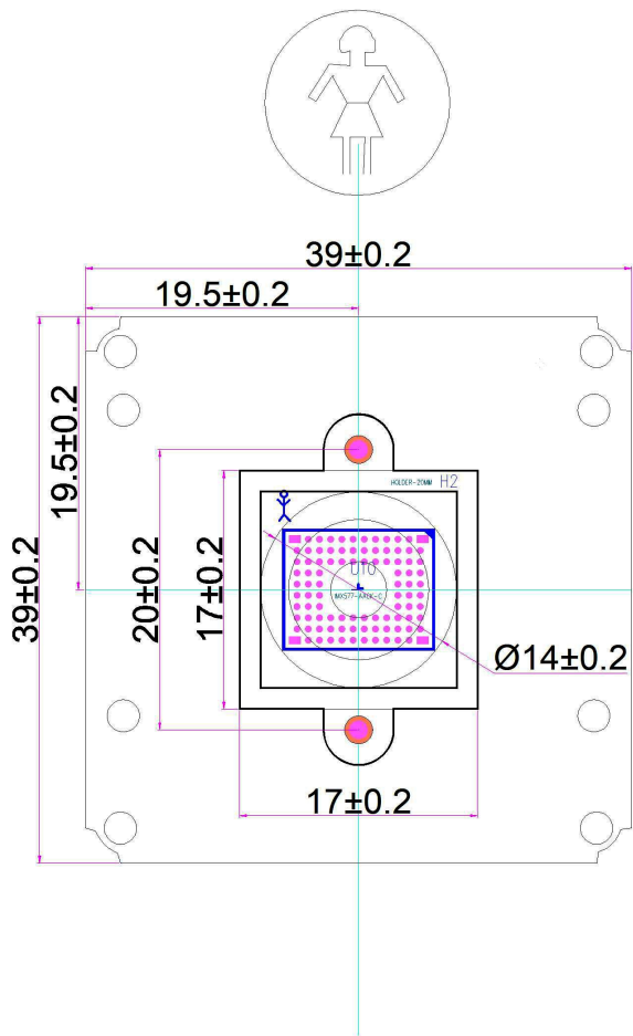
Top view
